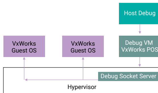
Figure 7. Platform debugger that supports system mode debugging of multiple VMs
